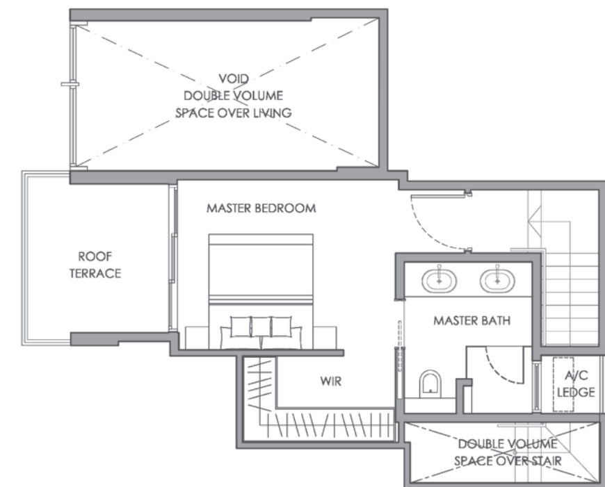
UPPER PLAN
